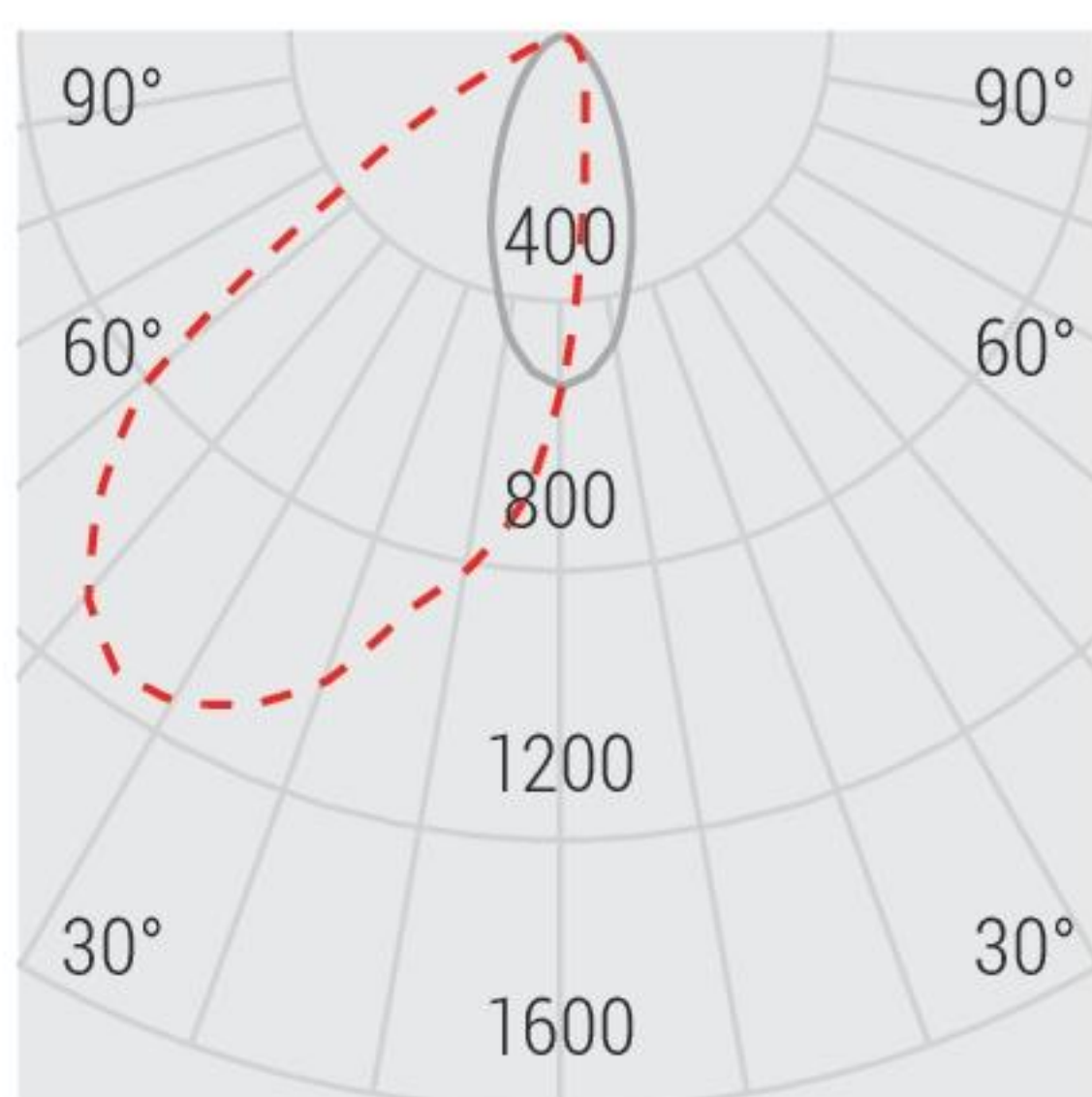
Photometric curve
