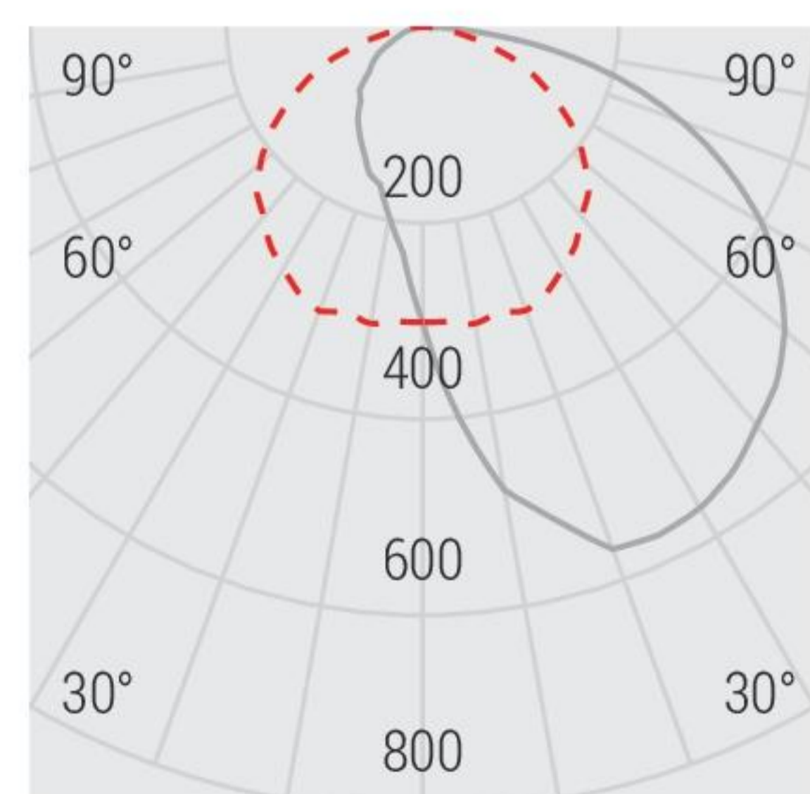
Photometric curve
