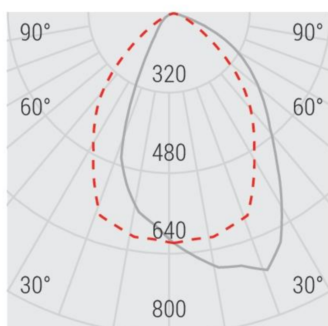
Photometric curve
