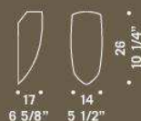
PERONI A1 1x70W E27 HSGSA/C alogeno chiara clear halogen 1x15W E27 FBT fluorescente fluorescent
