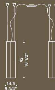
CARRÈ S2GD 2x70W E27 HSGSA/C alogeno chiara clear halogen 2x26W E27 FBT fluorescente fluorescent cavo elettrico 200 cm cables length 200 cm
