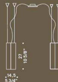
CARRÈ S2PD 2x70W E27 HSGSA/C alogeno chiara clear halogen 2x26W E27 FBT fluorescente fluorescent cavo elettrico 200 cm cables length 200 cm
