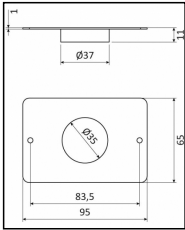
A814K0001KK Wall plaque
